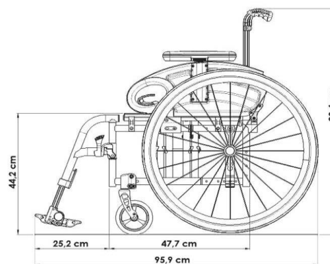
Setting of the chair above is: SD 400 mm and 24" wheel
